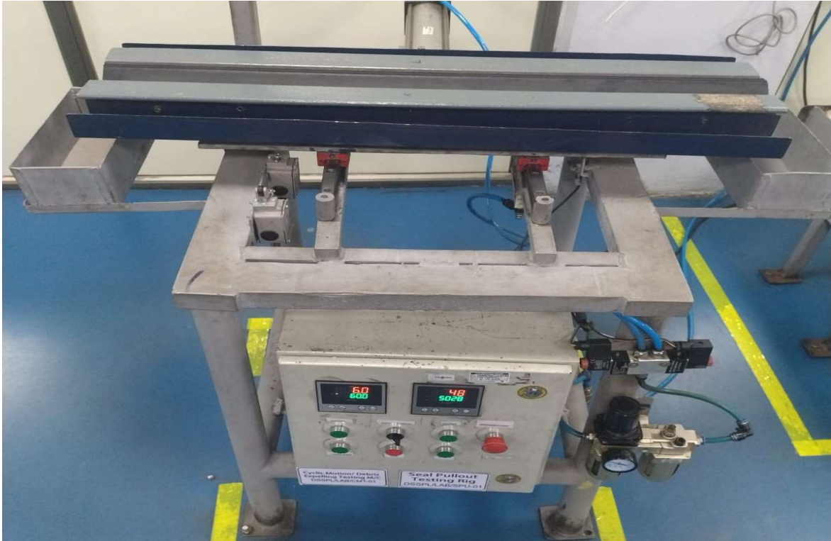
Expansion Joint Cyclic Motion, Seal Pull out & Debris Expelling Test facility
