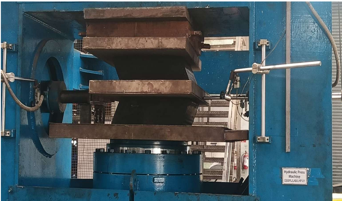
Elastomeric Bearing Shear Modules & Shear Bond Load Test Facility
